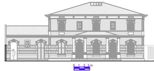
Elevation 03
